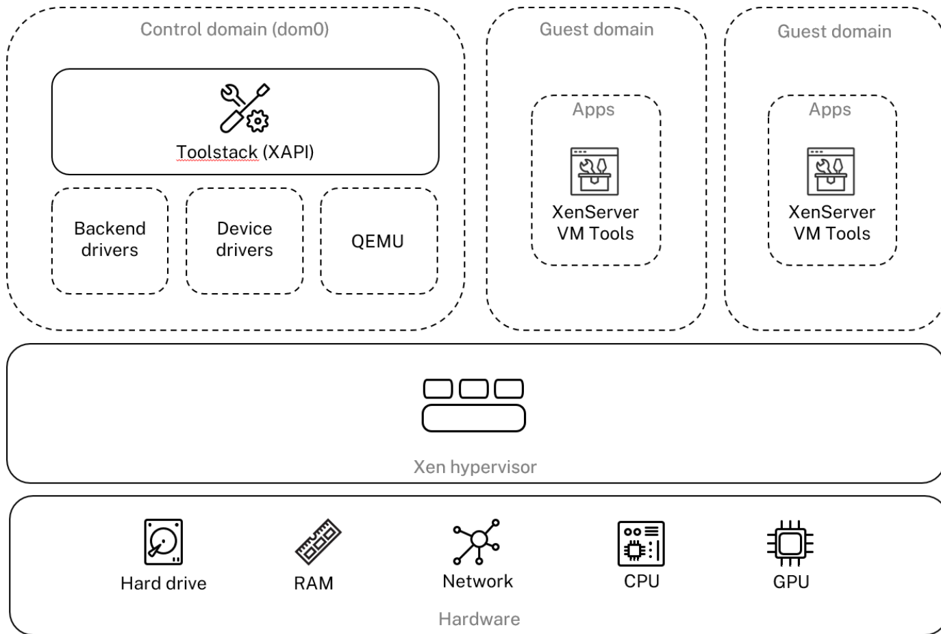
Architecture overview
