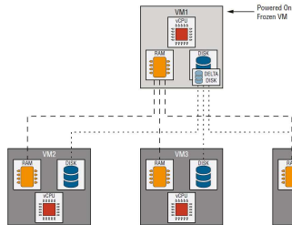
FIGURE 10.9 Frozen VMs will never have more than a single delta disk and can be cloned as many times as needed.
