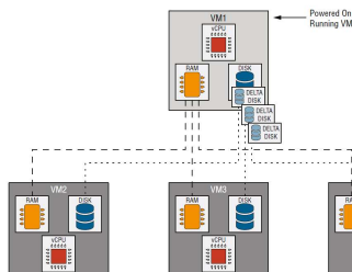
FIGURE 10.8 The instant-clone process for powered-on VMs creates a new delta disk on the source VM each time a clone is created.
